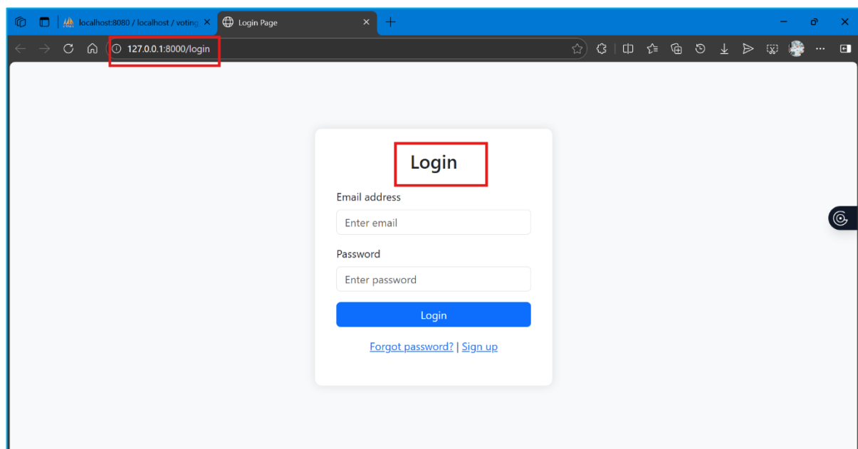
Figure 2.3 Login Option
