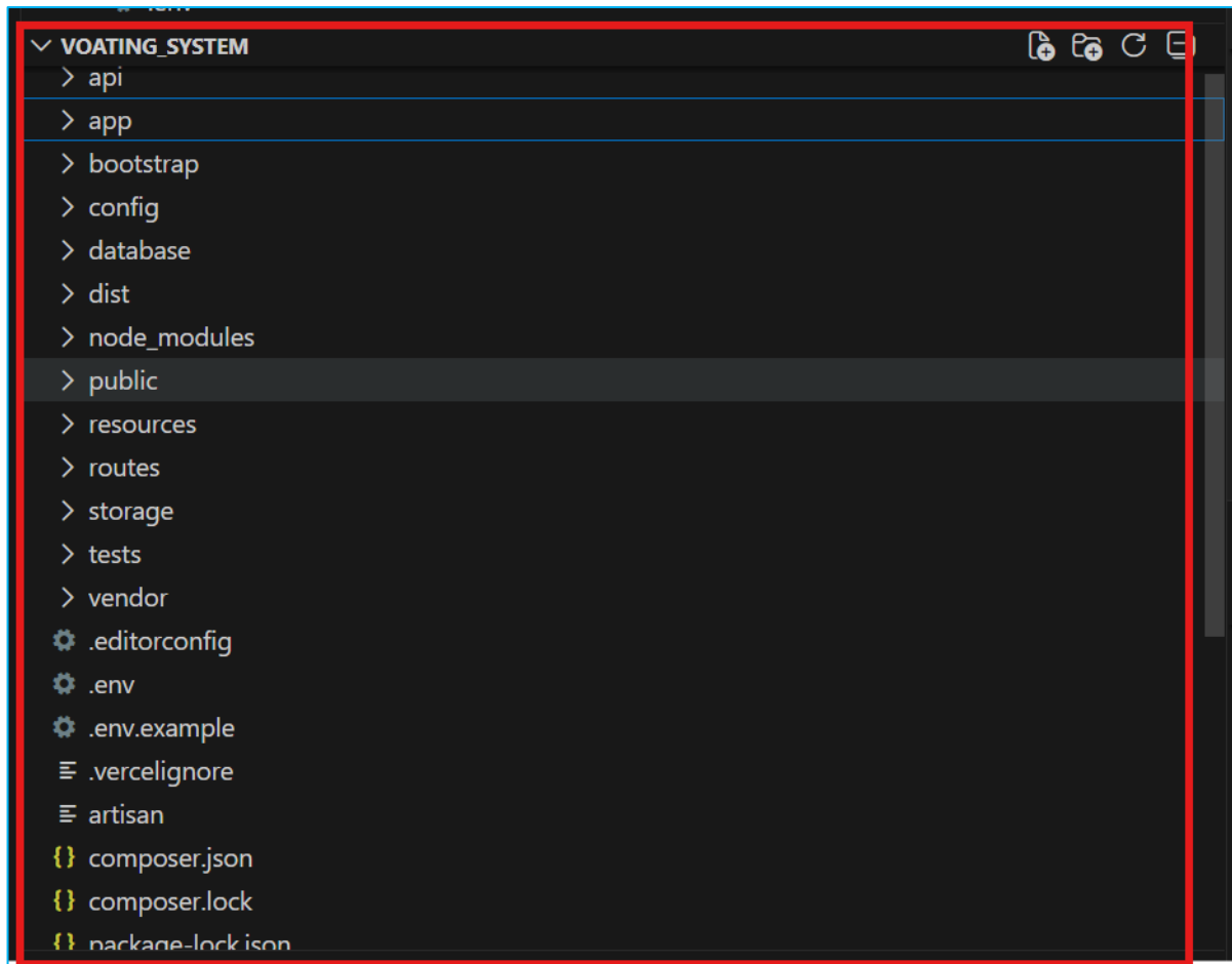
Figure 1 Project Structure
