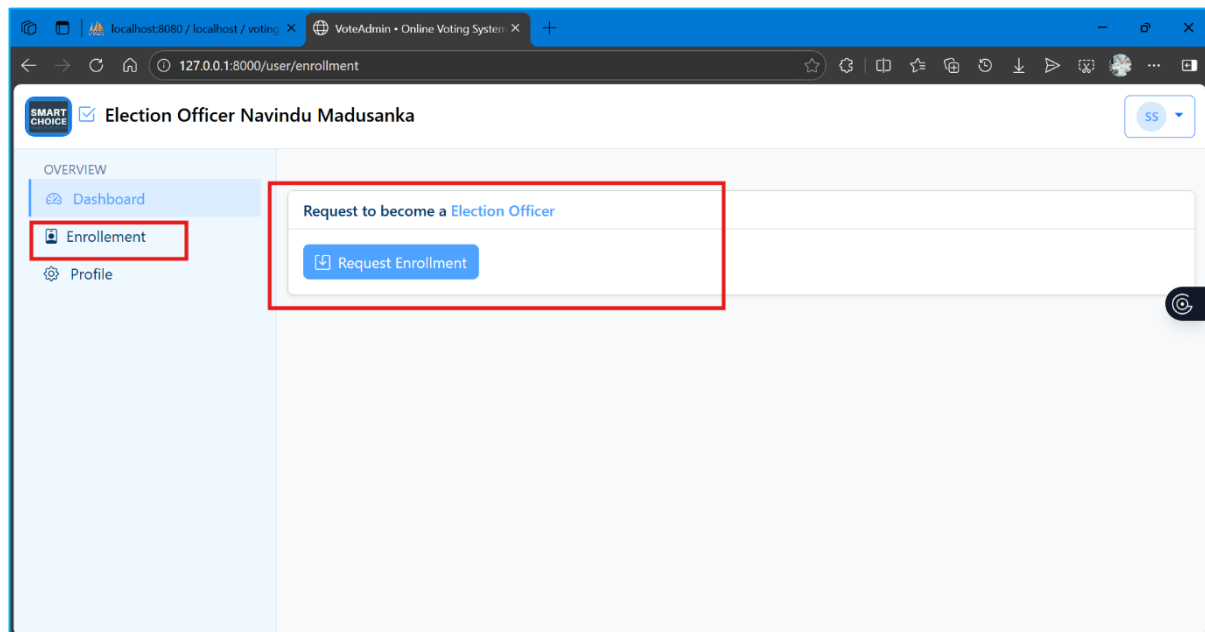
Figure 3.1 Enrollment Option
